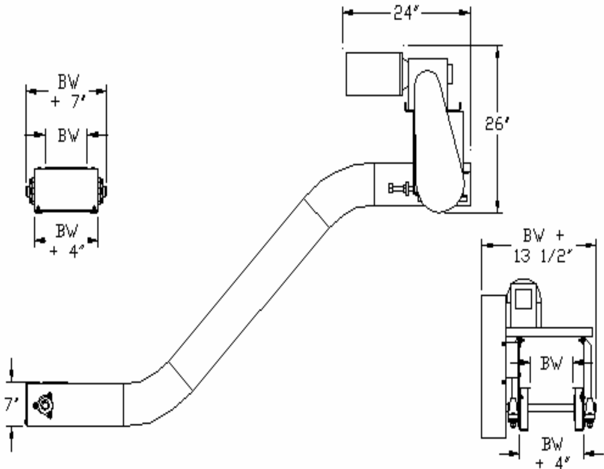
TOP MOUNT DRIVE
